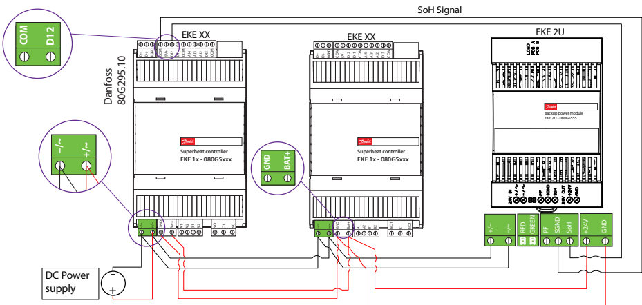
SHARING EKE 2U WITH 2 CONTROLLERS
