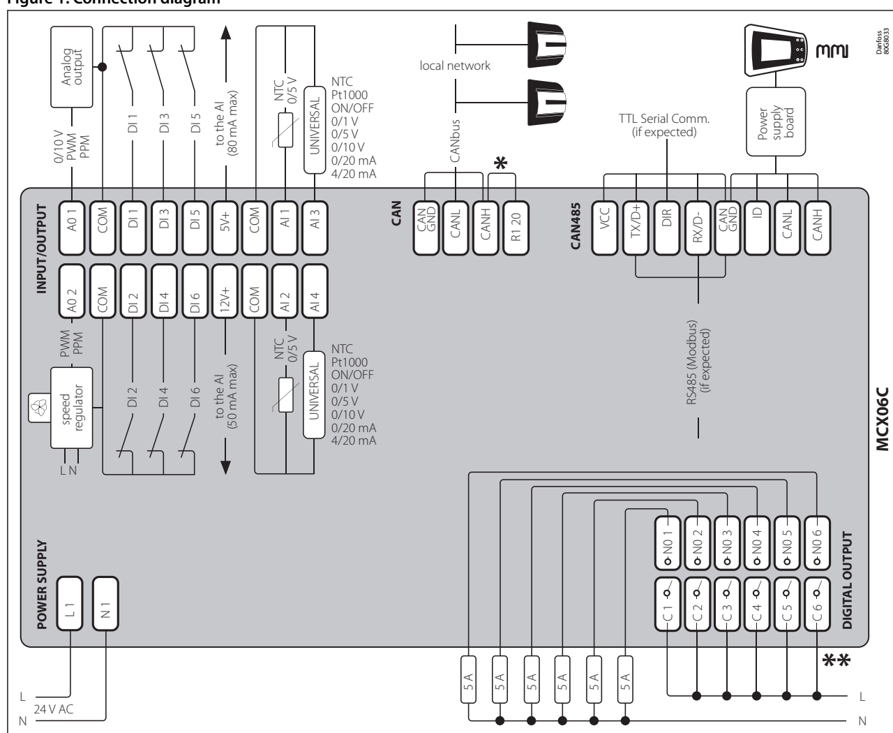
Figure 1: Connection diagram
