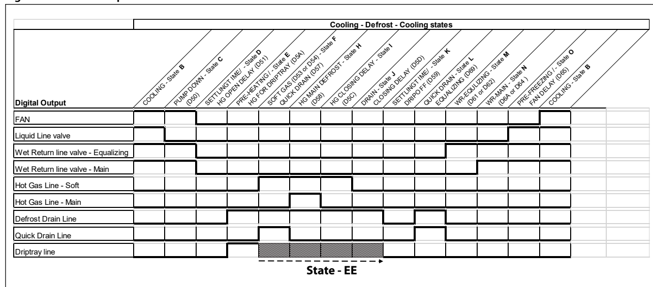
Figure 21: Defrost sequence
