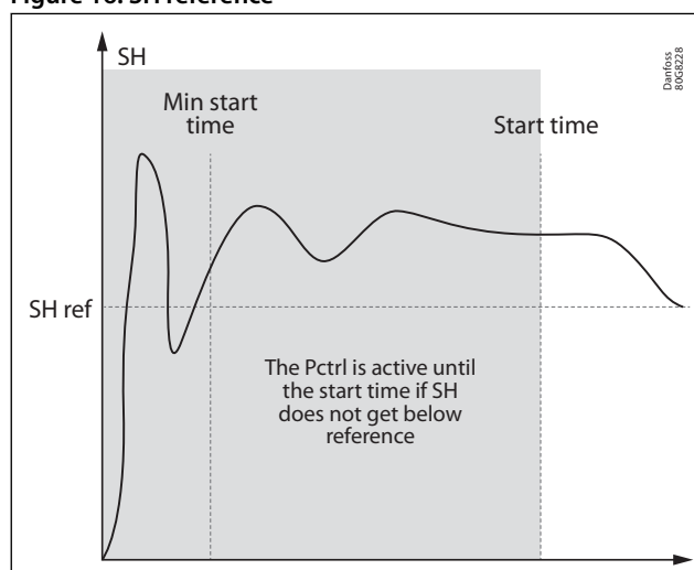
Figure 16: SH reference
