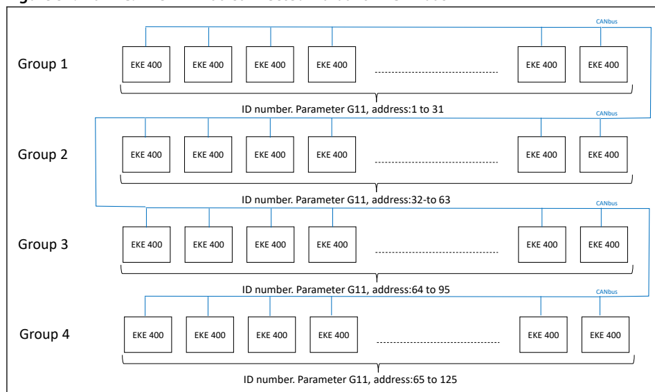
Figure 31: No PLC. Alle EKE 400 connected via built-in CANbus
