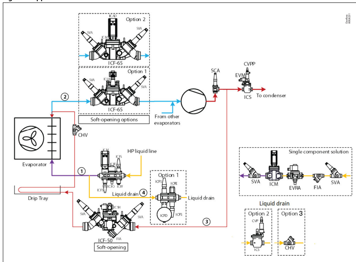
Figure 3: Application sketch
