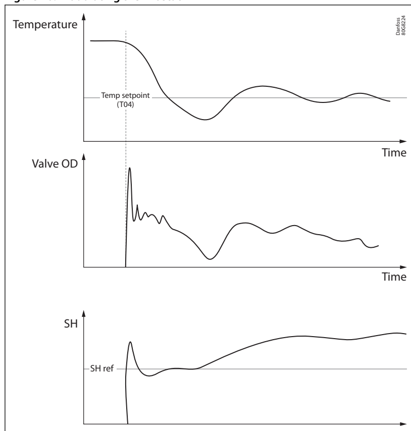
Figure 10: Modulating thermostat
