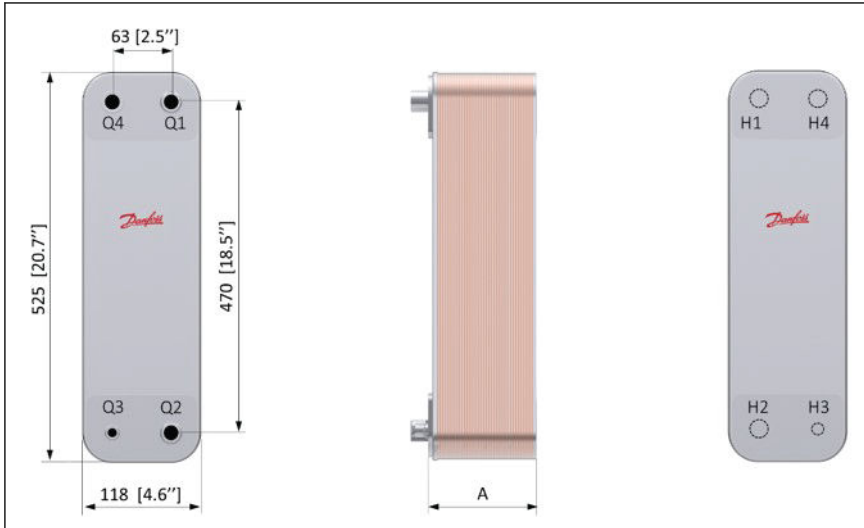
Figure 1: Dimensions
