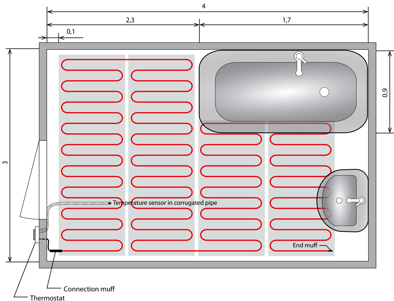
Fig. 1 – Example of heating mat installation in bathroom. All distances are in [m].
