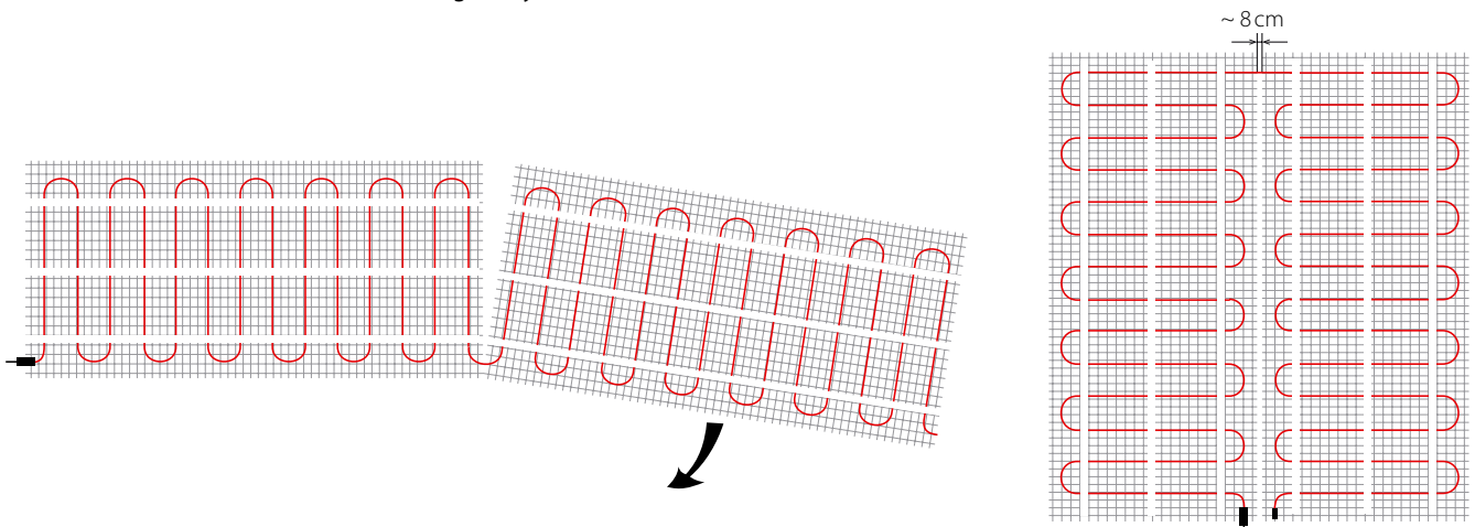
Fig. 9. The heating mats can be very easily adapted to the shape of the heated surface. Example above: placing ECmat 150T 50 x 300 cm on 100 x 150 cm.
