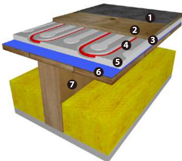
Fig. 22. Floor heating with Reflect insulated plates (EFCI Dry) on existing wooden floors
