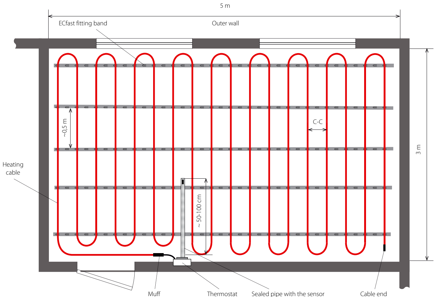
Fig. 2 - Example of heating cable installed in a room. Direct Floor Heating
