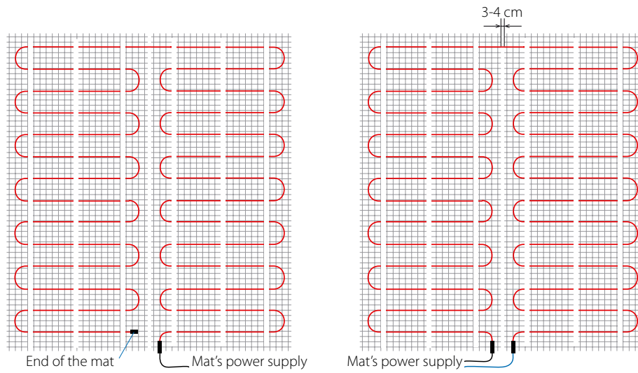
Fig. 7. Example of layout of a twin and single conductor heating mat.
