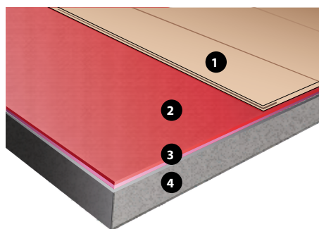
Fig. 16. Floor heating with ECdry on existing concrete subfloor
