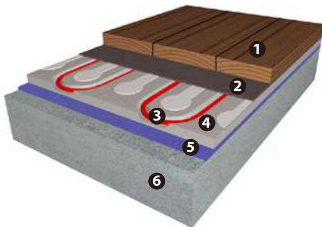
Fig. 21. Floor heating with Reflect insulated plates (EFCI Dry) on concrete floors
