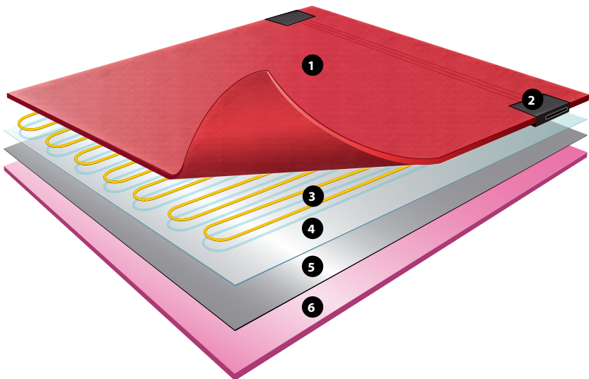
Fig. 15. ECdry heating element construction
