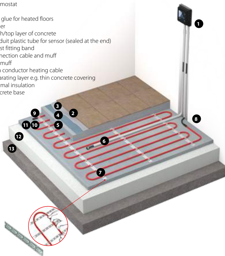
Fig. 4. Cable heating in concrete floor with cable fixed by ECfast fitting band.
