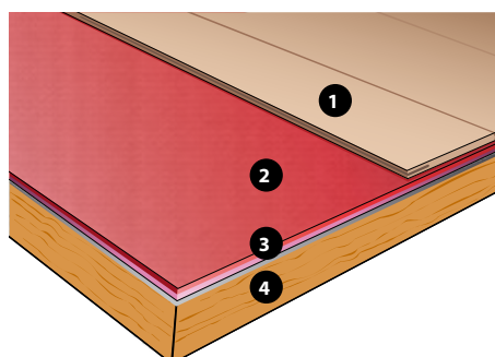
Fig. 17. Floor heating with ECdry on existing wooden subfloor
