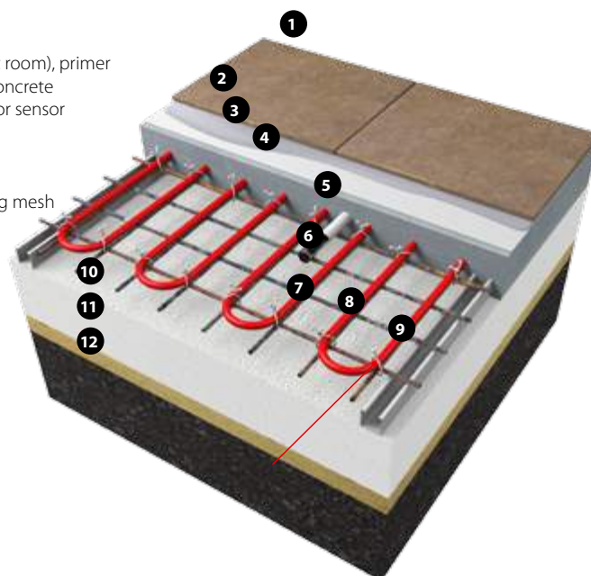
Fig. 5. Cable heating in concrete with cable fixed to reinforcement mesh by plastic cable ties.
