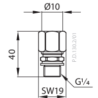
Compression fitting
