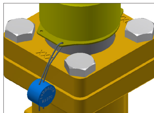
Example of marking ring, REG-SA
