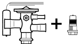
Thermostatic valve + Orifice
