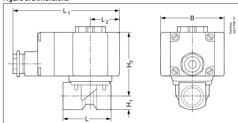
Figure 8: Dimensions
