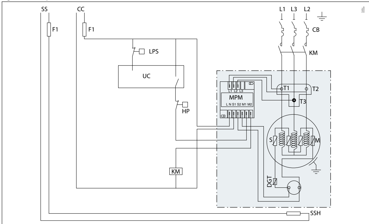
Figure 24: Compressor model CH290
