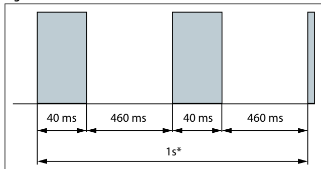
Figure 17: PTC Overheat
