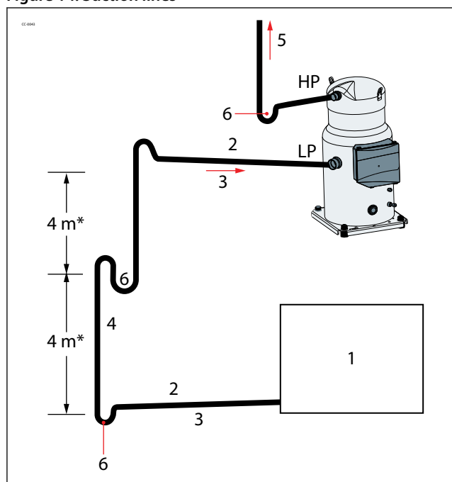
Figure 14: Suction lines
