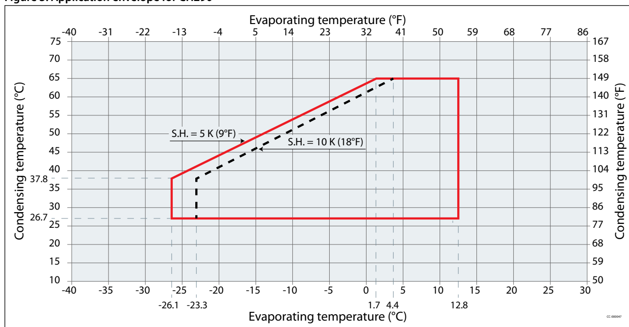
Figure 3: Application envelope for CH290
