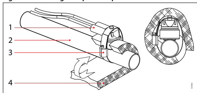
Figure 22: Discharge temperature protection
