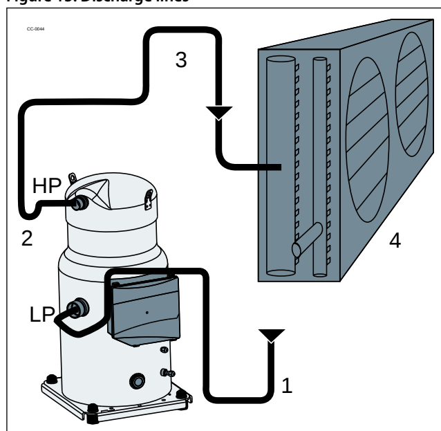
Figure 15: Discharge lines
