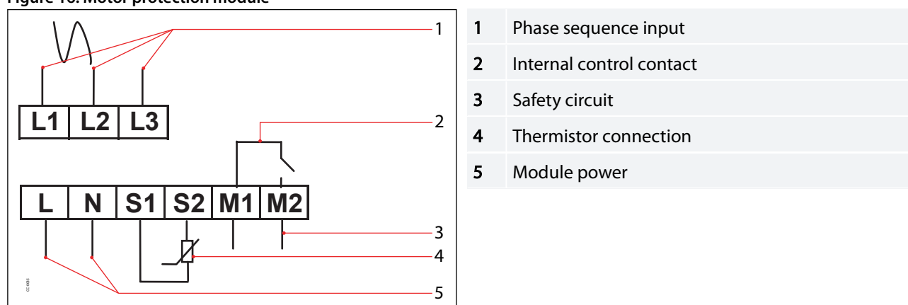
Figure 16: Motor protection module
