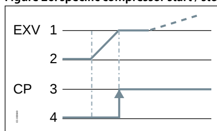
Figure 26: specific compressor start / stop control
