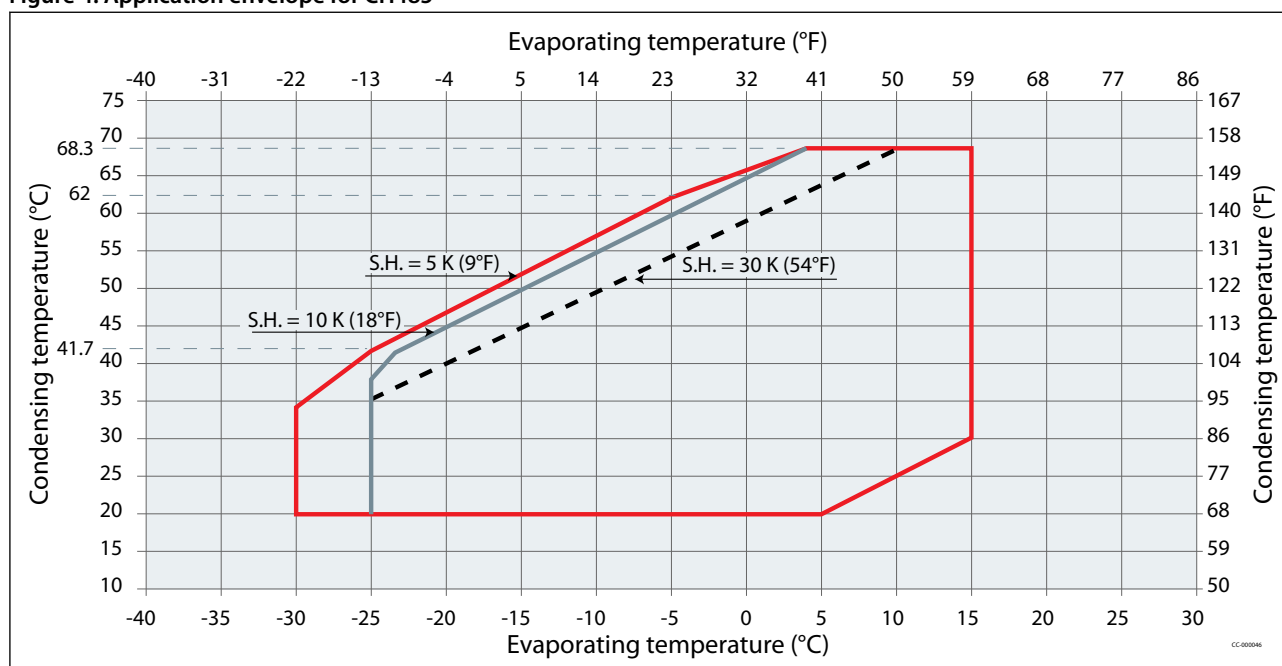
Figure 4: Application envelope for CH485
