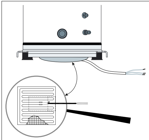
Figure 23: Sump heater
