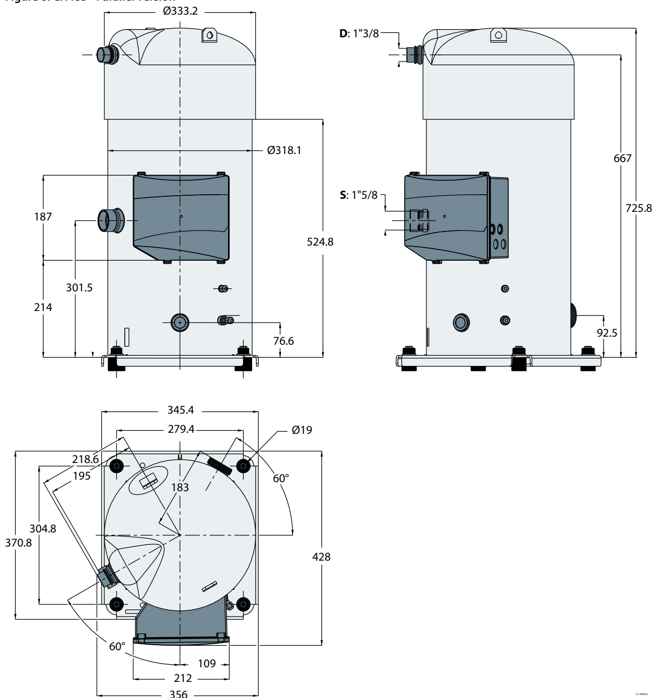
Figure 8: CH485 - Parallel version
