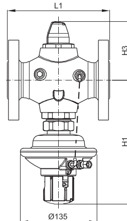
AVPQ (PN25) DN 32 - 50 \Delta p = 0.2 - 1.0
