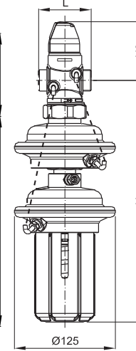
AVPQ 4 (PN25) DN 15 - 50 \Delta p = 0.2 - 1.0 \Delta p = 0.3 - 2.0
