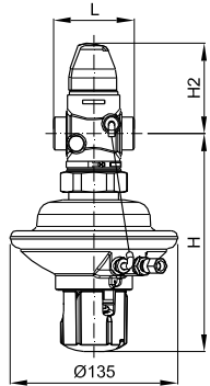
AVPQ (PN25) DN 15 - 50 \Delta p = 0.2 - 1.0
