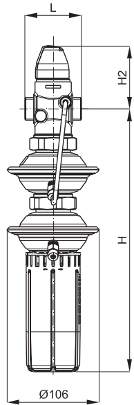
AVPQ (PN16) DN 15 - 32 \Delta p = 0.1 - 0.5 \Delta p = 0.2 - 1.0
