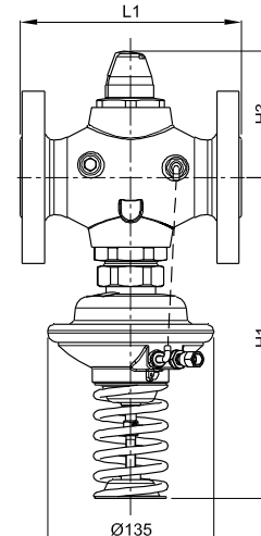
AVPQ (PN25) DN 32 - 50 \Delta p = 0.3 - 2.0
