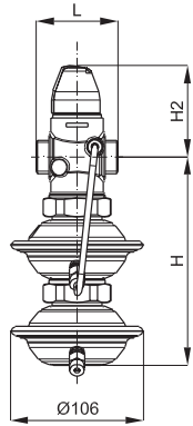
AVPQ-F (PN16) DN 15 - 32 \Delta p = 0.2 \Delta p = 0.3
