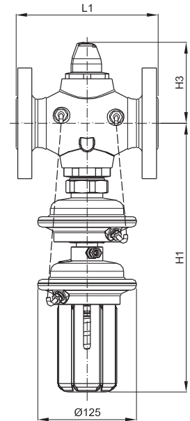
AVPQ 4 (PN25) DN 32 - 50 \Delta p = 0.2 - 1.0 \Delta p = 0.3 - 2.0
