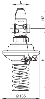
AVPQ (PN25) DN 15 - 50 \Delta p = 0.3 - 2.0
