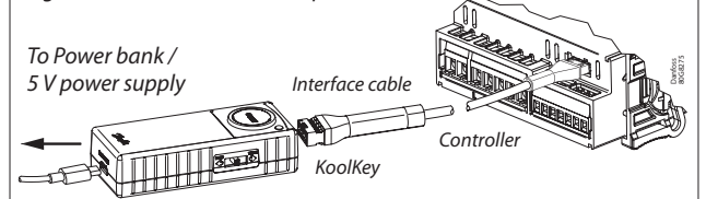
Fig. 4: Controller without main power
