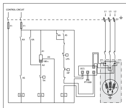
Wiring diagram without pump-down cycle
